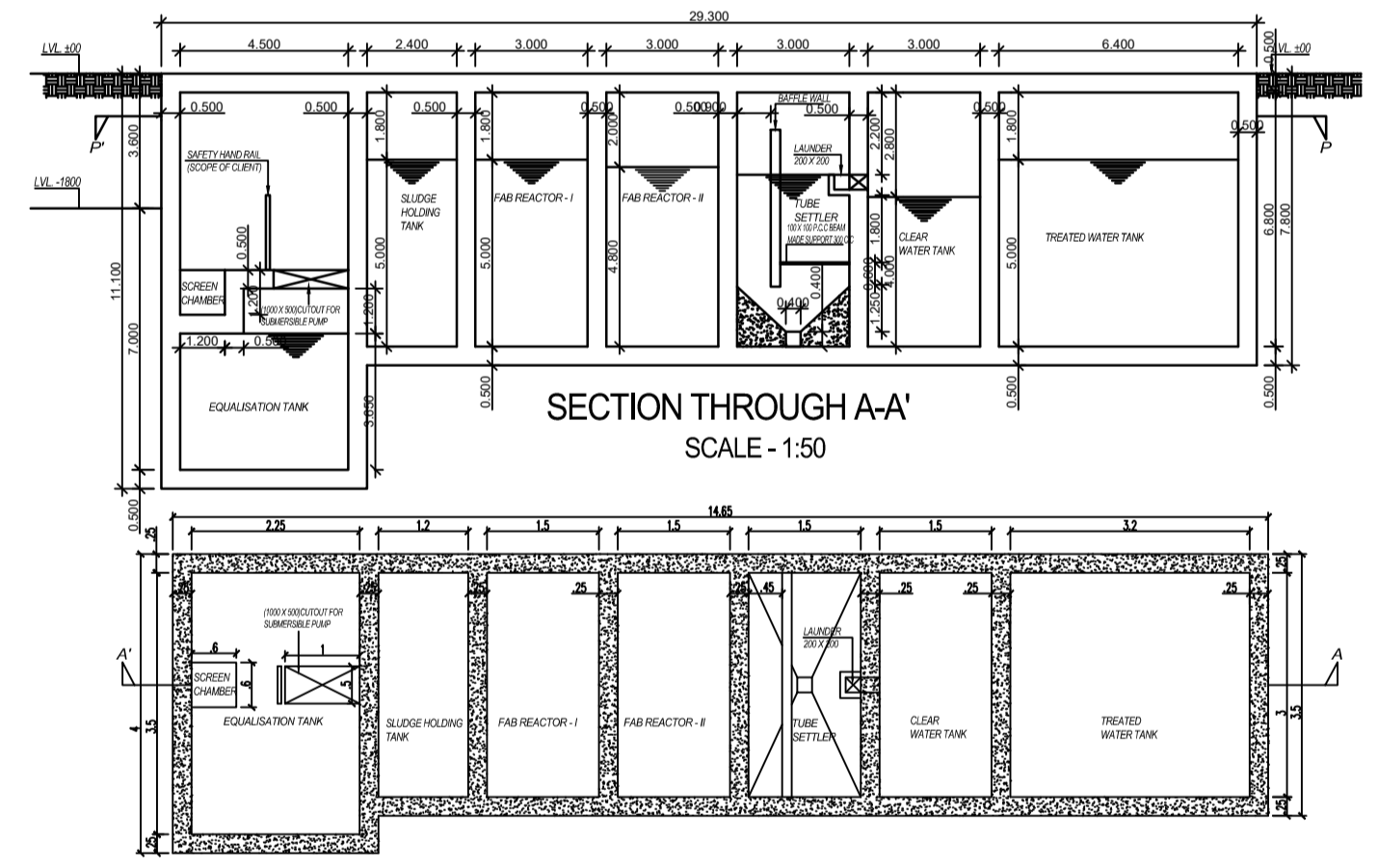
SEWAGE TREATMENT PLANT PLAN AT LEV. P-P' SCALE - 1:50
